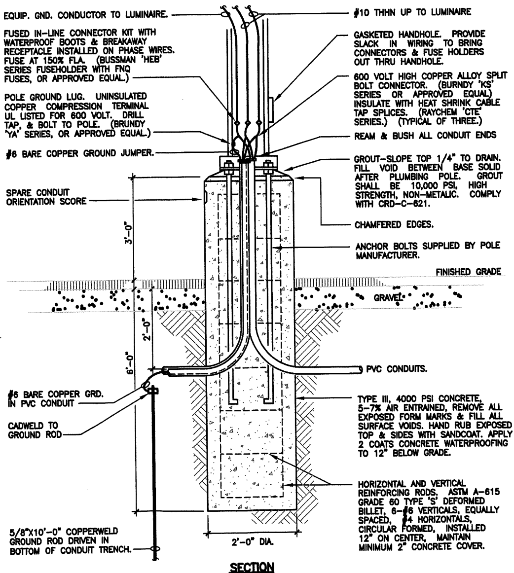
1 36° POLE BASE DETAIL SU1.01 NO SCALE
